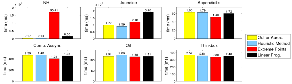
Fig. 3. Evaluation times for the IIDs in Tab. 1 and relative duration w.r.t. the evaluation of the corresponding IDs
