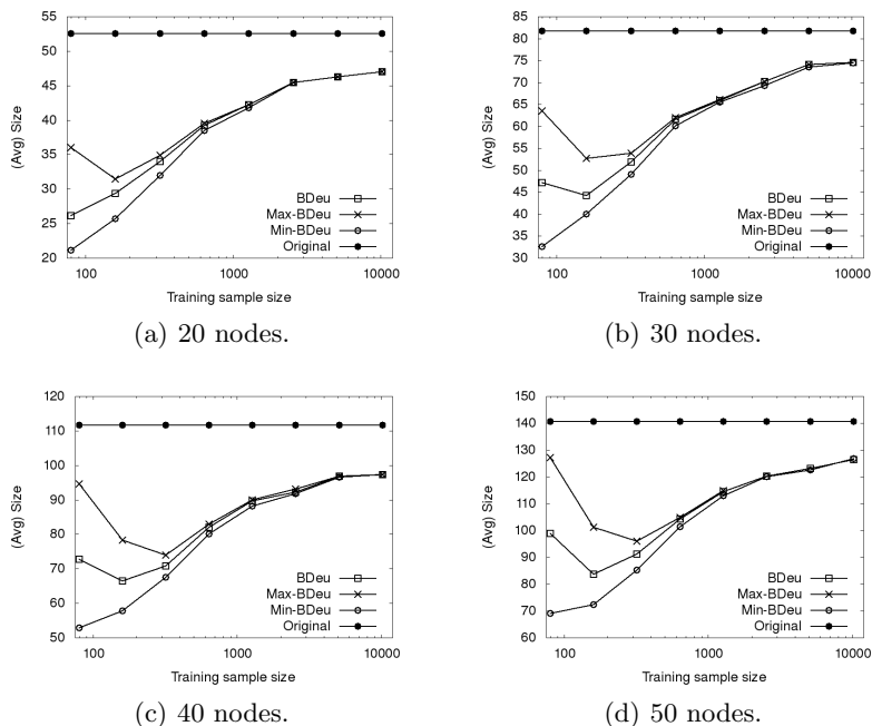
Fig. 4. Comparison on average total number of arcs in the learned networks from different score functions. The graphs feature BDeu (square points), Max-BDeu (cross points), Min-BDeu (circle points), Original (bullet points). The points in the curves correspond to the total number of arcs in the graphs of learned networks.
