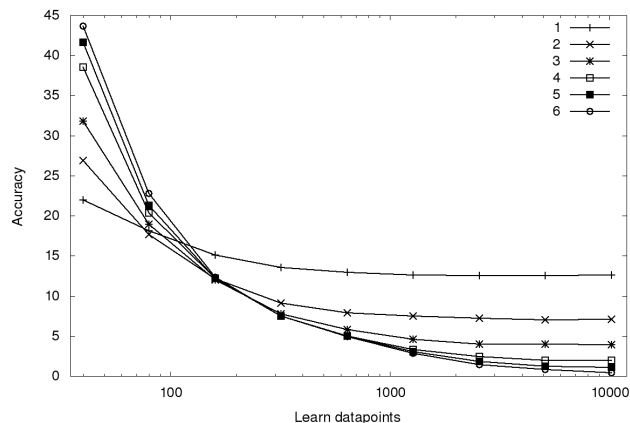
Fig. 7. Average accuracy curves of learned networks from data of randomly generated Bayesian networks with 20 nodes. Different curves represent the result of inferred networks under different parent set size limits during learning: maximum of one parent up to maximum of six parents.
