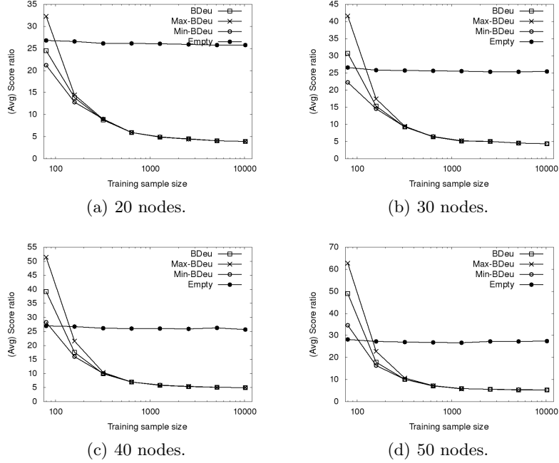
Fig. 1. Comparison on average computed accuracy score among networks learned from different score functions. The graphs feature BDeu (square points), Max-BDeu (cross points), Empty (bullet points), Min-BDeu (circle points). Each curve of the graph corresponds to the average over random networks used for sampling the data. The points in those curves correspond to the accuracy score for different training data sample size.
