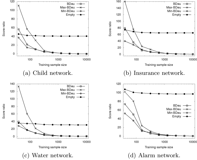
Fig. 2. Comparison on computed accuracy score among networks learned from different score functions using data generated with well-known Bayesian networks. The graphs feature BDeu (square points), Max-BDeu (cross points), Min-BDeu (circle points), Empty (bullet points). The points in the curves correspond to the accuracy score for different training data sample size.
