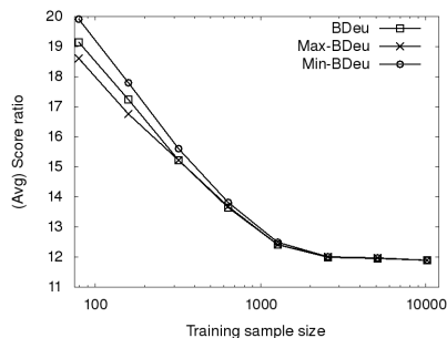
Fig. 5. Comparison on average computed accuracy score among networks learned from different score functions. The graphs feature BDeu (square points), Max-BDeu (cross points), Min-BDeu (circle points). The structure of the networks is learned with the given training data sample size, while the parameters are learned with a fixed big training data sample.
