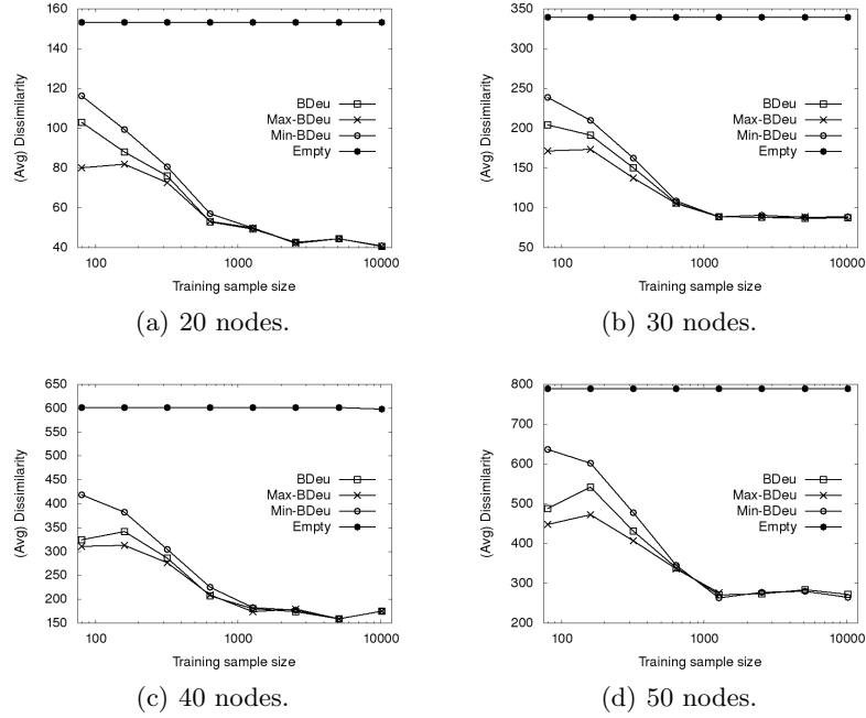
Fig. 3. Comparison on average computed dissimilarity between true and learned networks using different score functions. The graphs feature BDeu (square points), Max-BDeu (cross points), Min-BDeu (circle points), Empty (bullet points). The points in the curves correspond to the total number of mismatches between the moral graph of true and learned networks.
