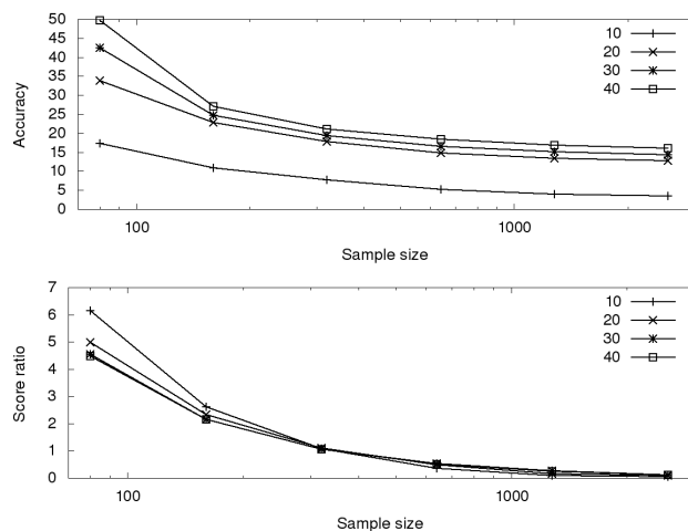
Fig. 6. Curves for accuracy score (upper graph) and sensitivity measure as ratio of Max- and Min-BDeu (lower graph) for inferred networks learned from training data of different sizes using randomly generated Bayesian networks with 10 to 40 nodes.
