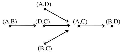
Figure 1. An example set-based weighted graph. The sets for the edges are specified separately by intervals that in two cases degenerate to real numbers.
