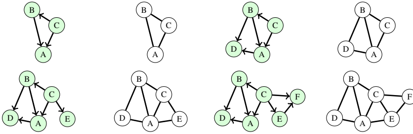
Fig. 4 Example of a treewidth-bounded DAG ( k=2 ) being built iteratively. On the left, the DAG at each step (green nodes) is presented, and on the right the resulting k -tree (white nodes). We start with the variables \{A, B, C\} and we add the remaining ones one at a time ( D, E and F ).
