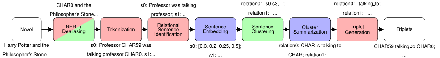
Figure 1: The workflow of the triplet generation process, with relation clustering.
